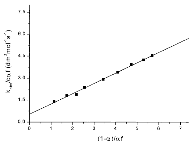
Figure 3. Using the Acree equation [Eqn. (2)] to determine k_i and k_{ip} for the substrate ( 2 ) with the salt KCl-Krypto
