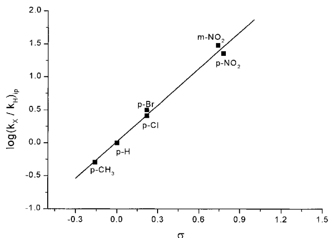
Figure 5. Hammett equation [Eqn. (3)] for the ion pair rate constants, k_{ip} , with \text{NBu}_4\text{Cl}
