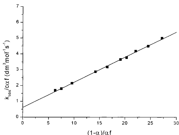
Figure 2. Using the Acree equation [Eqn. (2)] to determine k_i and k_{ip} for the substrate ( 2 ) with the salt \text{NBu}_4\text{Cl}
