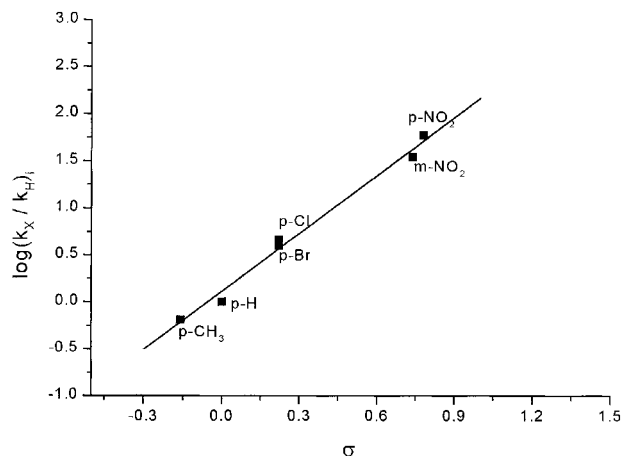
Figure 4. Hammett equation [Eqn. (3)] for the ion rate constants, k_i , with \text{NBu}_4\text{Cl}
