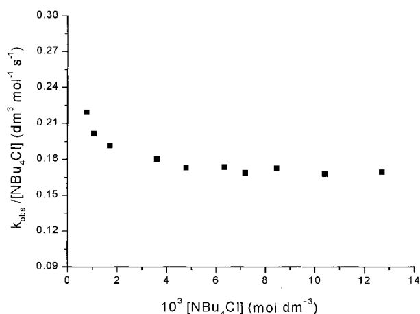
Figure 1. Plot of k_{\text{obs}}/[\text{NBu}_4\text{Cl}] versus [\text{NBu}_4\text{Cl}] for the reaction with methyl m -nitrobenzenesulphonate
